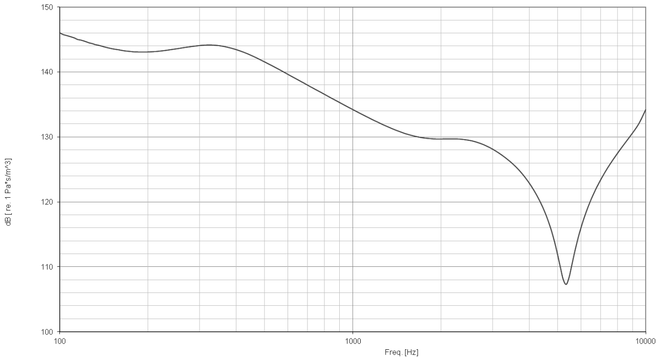
Acoustic input impedance of the RA0039
